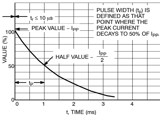
Figure 4. Pulse Waveform
