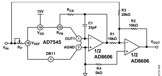
Figure 56. Bipolar Operation
