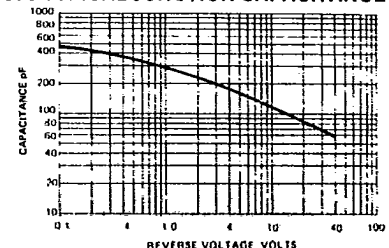
FIG. 5-TYPICAL JUNCTION CAPACITANCE
