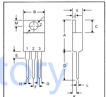
TO-220AB
