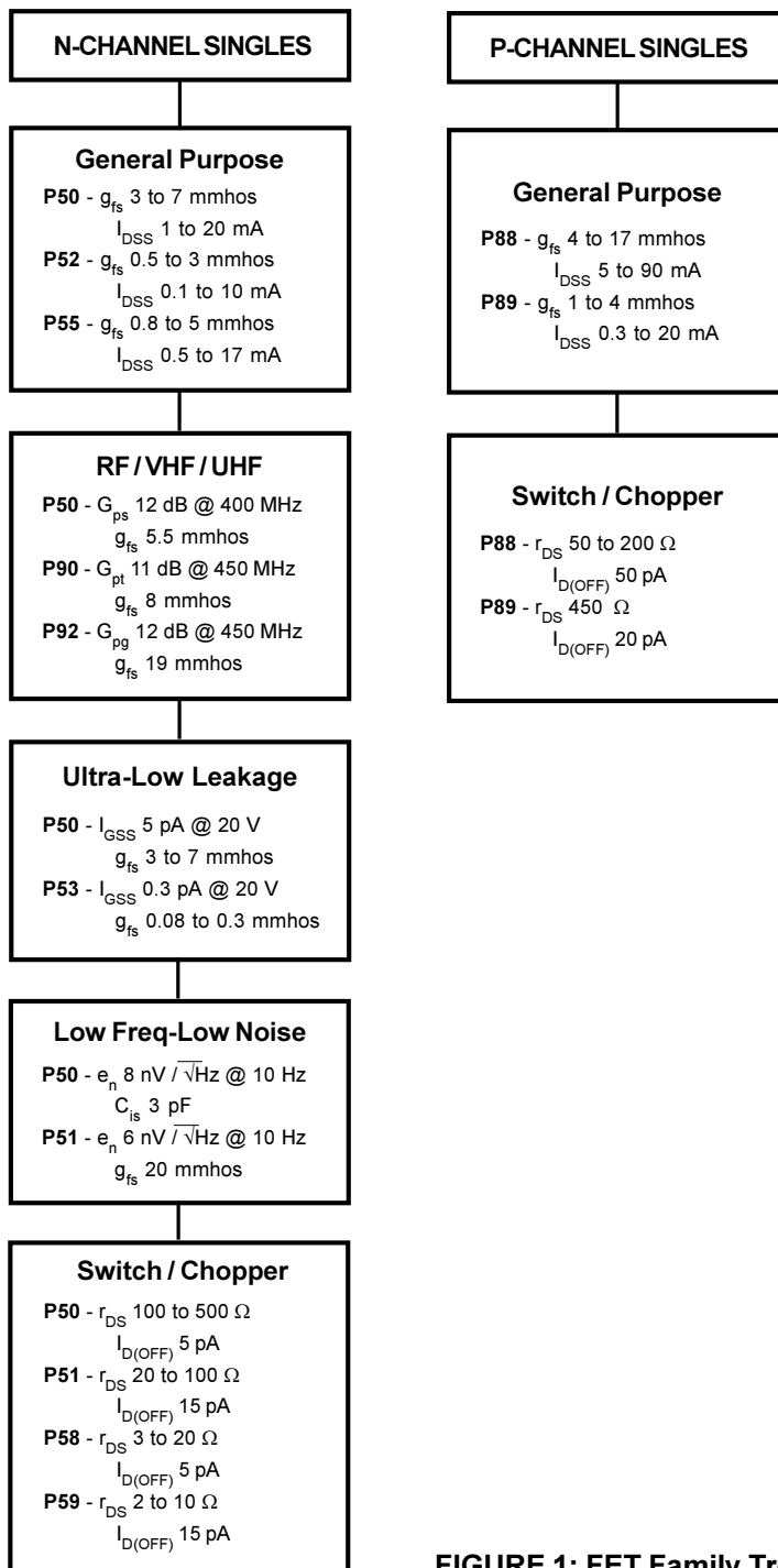
FIGURE 1: FET Family Tree
