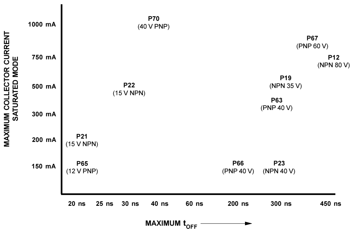
FIGURE 1: Transistor Processes for High Speed Switching
