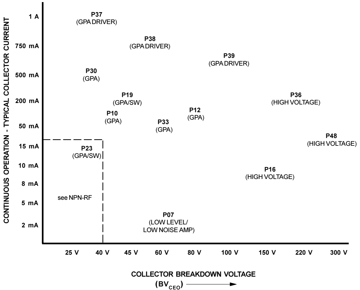
FIGURE 1: Transistor Processes By Dynamic Capability
