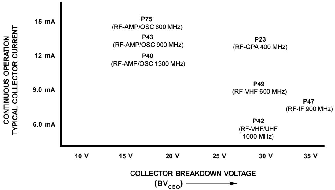
FIGURE 1: Transistor Processes For Radio Frequency
