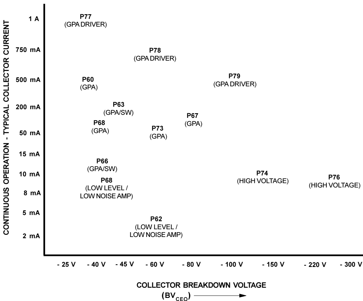
FIGURE 1: Transistor Processes By Dynamic Capability
