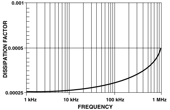
TYPICAL PARAMETER C0G (NP0) CHANGE OF CAPACITANCE WITH FREQUENCY - NP0
