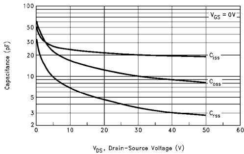
FIGURE 9. Capacitance vs Drain-Source Voltage
