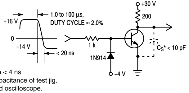
Figure 2. Turn-Off Time
