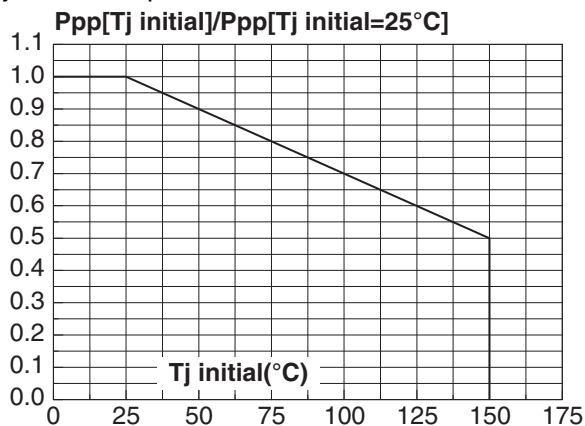
Fig. 2: Peak power dissipation versus initial junction temperature.
