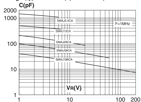
Fig. 5-2: Capacitance versus reverse applied voltage (typical values) (SMAJxxCA).
