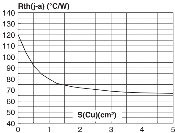
Fig. 8: Thermal resistance junction to ambient versus copper surface under each lead (printed circuit board FR4 e(Cu)=35µm).
