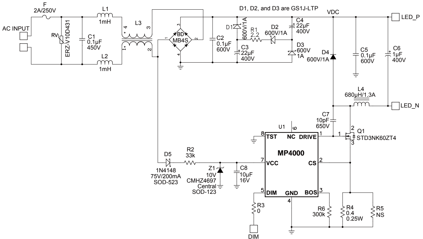
Figure 2 Reference Design Circuit: Universal Input, 3~12W LED Lighting Solution
