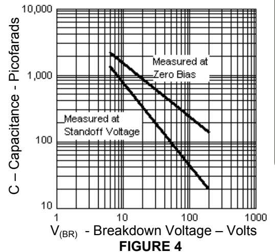
Typical Capacitance vs. Breakdown Voltage
