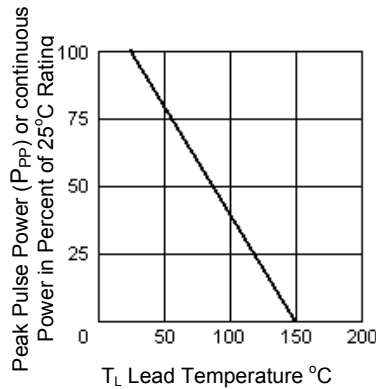
FIGURE 3 Derating Curve
