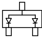
Figure 2, Common Anode
