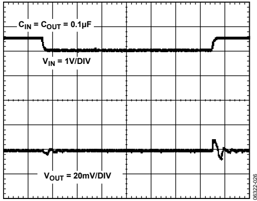
Figure 26. Line Transient Response, V_{OUT} = 0.5 V
