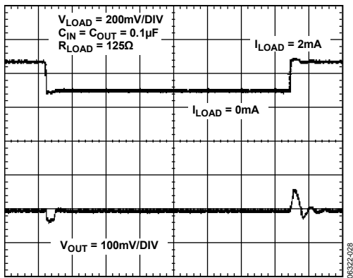
Figure 28. Load Transient Response (Sink), V_{OUT} = 0.5 V
