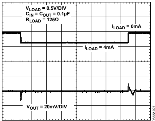
Figure 27. Load Transient Response (Source), V_{OUT} = 0.5 V
