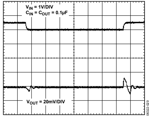
Figure 29. Line Transient Response, V_{OUT} = 1 V
