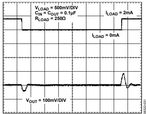
Figure 31. Load Transient Response (Sink), V_{OUT} = 1 V
