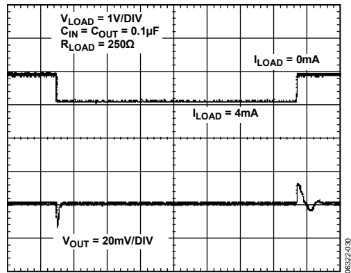
Figure 30. Load Transient Response (Source), V_{OUT} = 1 V
