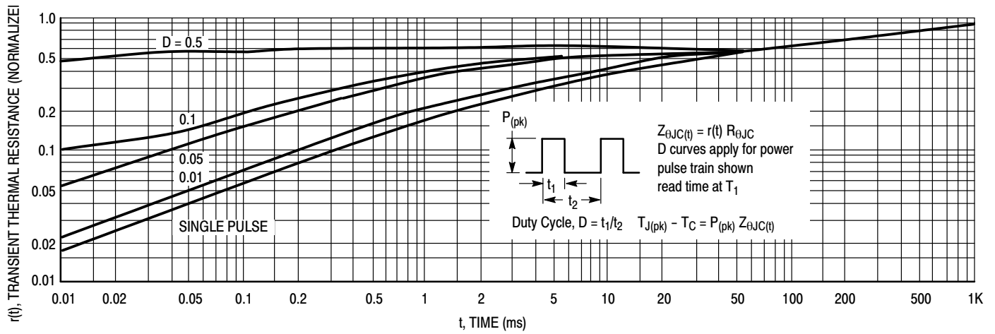
Figure 5. Thermal Response
