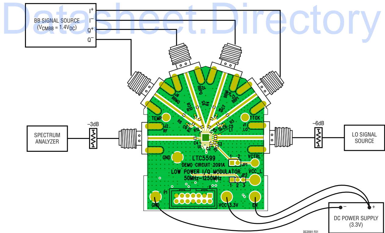
Figure 1. Test Setup for RF Performance Measurements
