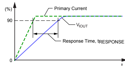
Figure 5: Response Time ( t_{\text{RESPONSE}} )
