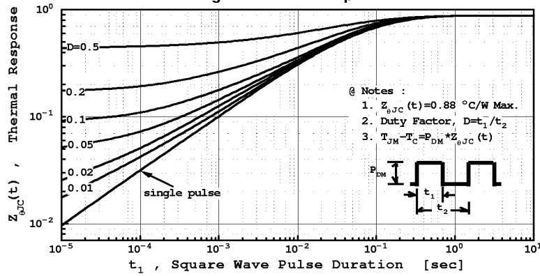
Fig 11. Thermal Response
