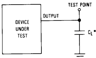
Figure 4. Test Circuit
