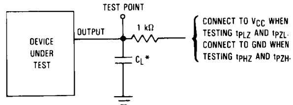
Figure 5. Test Circuit
