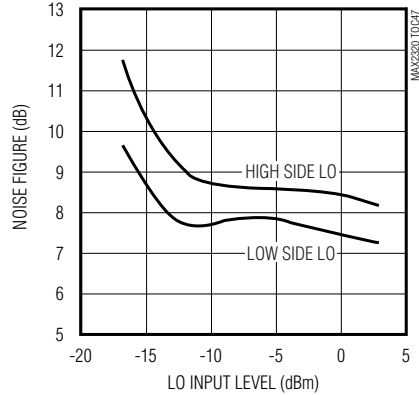
PCS-BAND HGGL MIXER NOISE FIGURE vs. LO INPUT LEVEL
