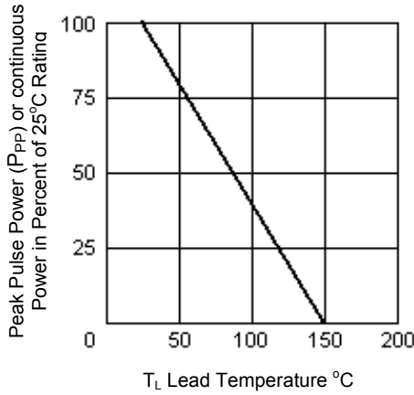
FIGURE 3 - Derating Curve
