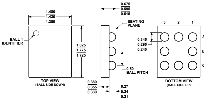
Figure 61. 8-Ball Wafer Level Chip Scale Package [WLCSP] (CB-8-1) Dimensions shown in millimeters
