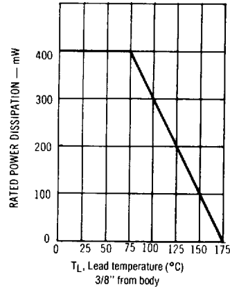
FIGURE 3 POWER DERATING CURVE
