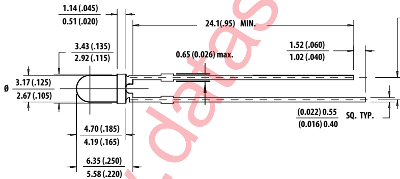
Figure A. T-1 package.
