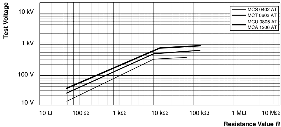
Pulse load rating in accordance with EN 60115-1 clause 4.27; 10 μs/700 μs; 10 pulses at 1 min intervals; for permissible resistance change 0.5 %
