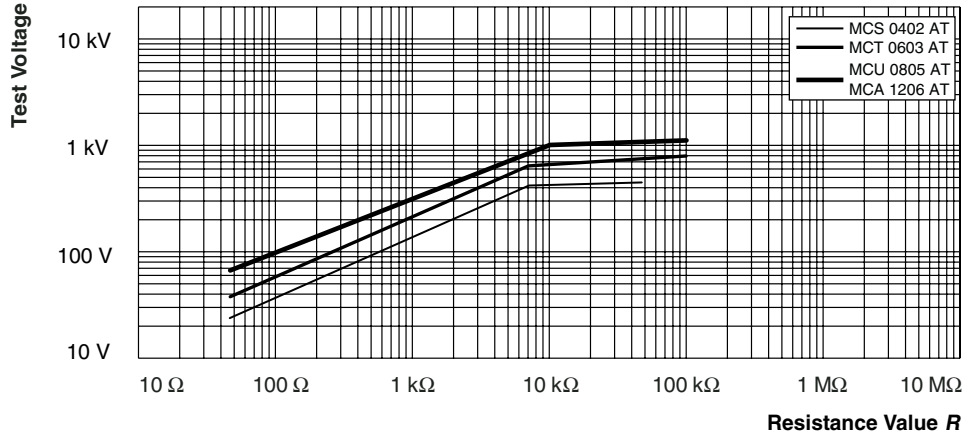
Pulse load rating in accordance with EN 60115-1 clause 4.27; 1.2 μs/50 μs; 5 pulses at 12 s interval; for permissible resistance change 0.5 %
