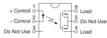
AC/DC Configuration
