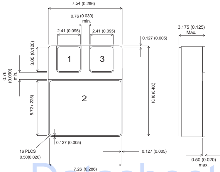
SMD0.5 (TO276AA)
