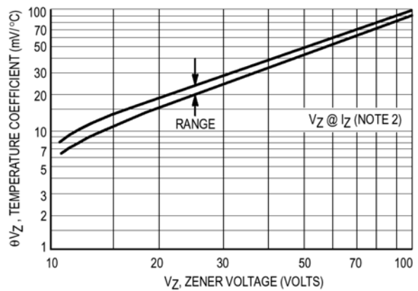
Figure 3. Temperature coefficients
