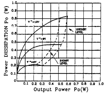
Power Dissipation vs. Output Power (RL=8Ω)
