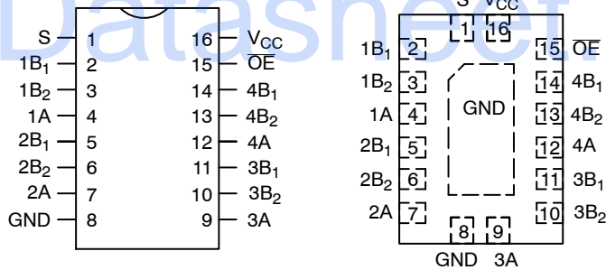
Figure 1. 16-Lead Pinout Diagrams
