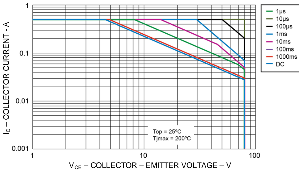
Maximum Safe Operating Area @ T_C = 25\text{ }^\circ\text{C}
