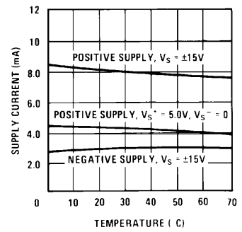
Supply Currents
