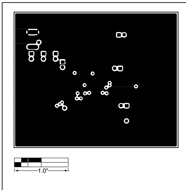
Figure 7. MAX2320/21/22/24/26/27 EV Kits PC Board Layout—Ground Plane 2
