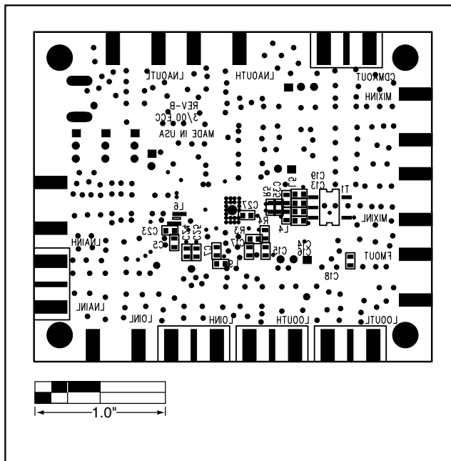
Figure 5. MAX2320/21/22/24/26/27 EV Kits Component Placement Guide—Solder Side
