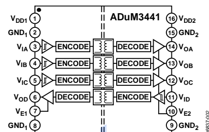
Figure 2. ADuM3441 Functional Block Diagram
