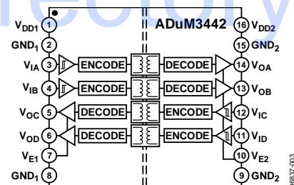
Figure 3. ADuM3442 Functional Block Diagram
