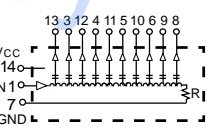
A1410 Schematic
