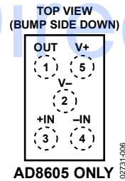
Figure 3. 5-Bump MicroCSP (CB Suffix)
