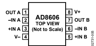
Figure 2. 8-Lead SOIC (R Suffix)
