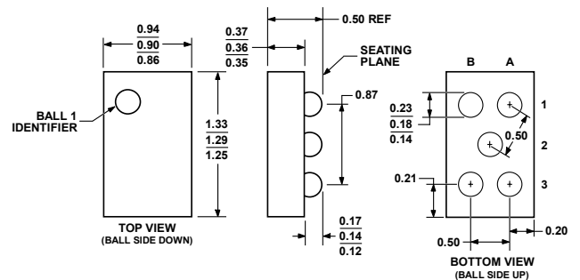
Figure 62. 5-Bump 2 x 1 x 2 Array MicroCSP [WLCSP] (CB-5) Dimensions shown in millimeters
