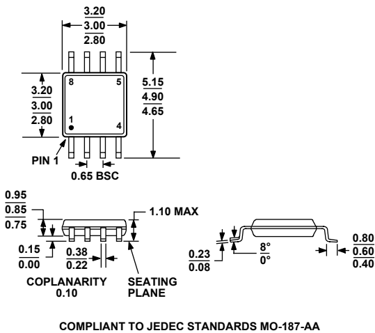
Figure 59. 8-Lead Mini Small Outline Package [MSOP] (RM-8) Dimensions shown in millimeters
