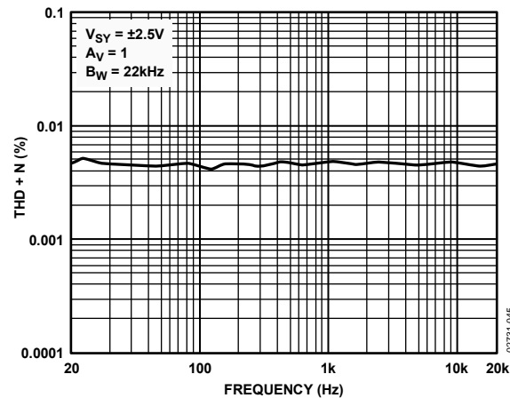
Figure 45. THD + N
