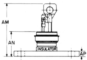
ISOLATED TO-3 FLANGE TYPE 4
