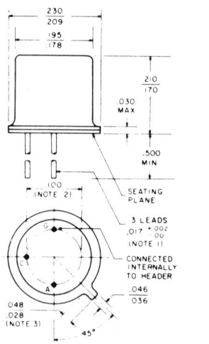
DIMENSIONS WITHIN JEDEC OUTLINE TO-18
