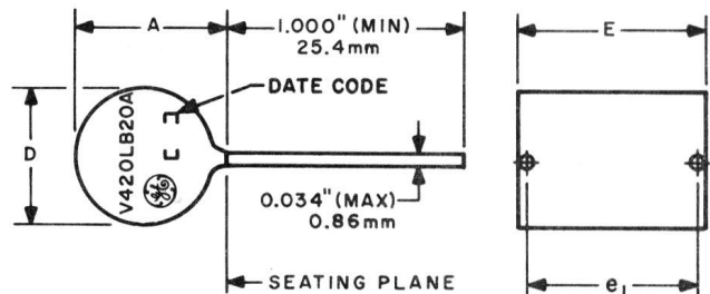
"LB" CONFIGURATION
