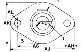
ISOLATED STUD TYPE 3
