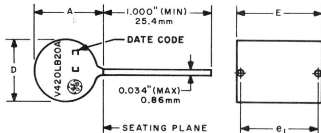
"LB" CONFIGURATION
