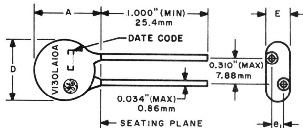
"LA" CONFIGURATION
