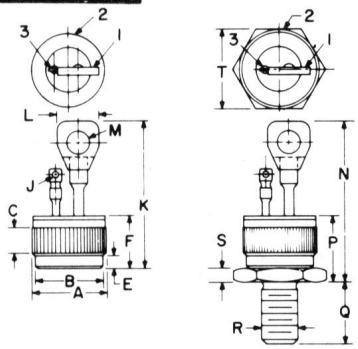
PRESS-FIT
