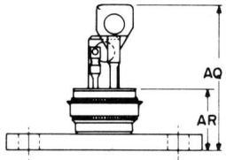
NON-ISOLATED TO-3 FLANGE TYPE 5
