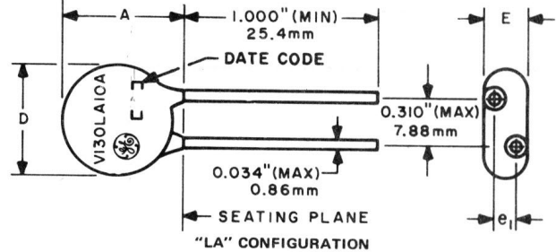
"LA" CONFIGURATION
