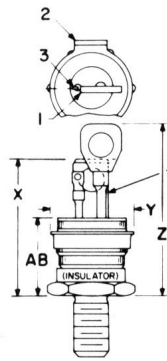
ISOLATED STUD TYPE 2
