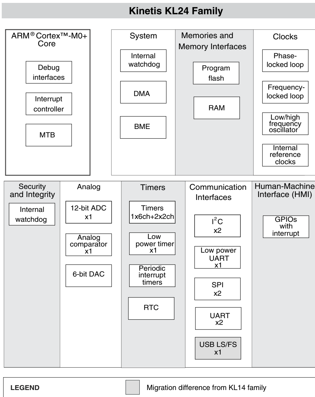
Figure 2. KL24 family block diagram
