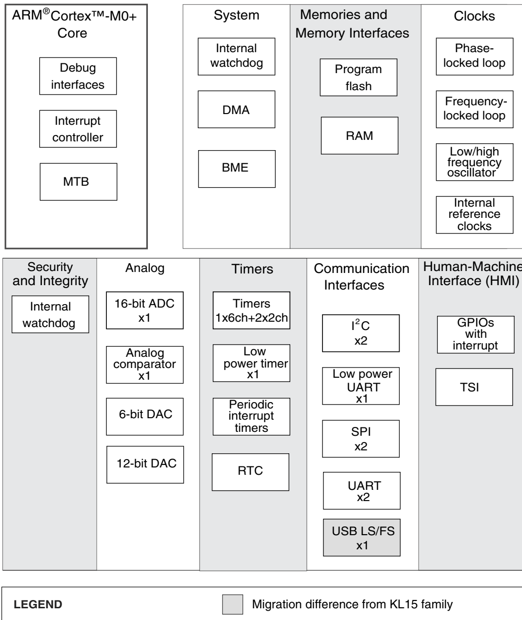
Figure 3. KL25 family block diagram
