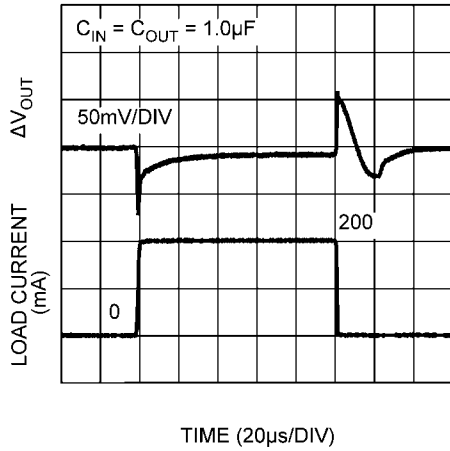
Load Transient Response. V_{OUT} = 2.8\text{V}
