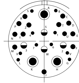
J20 10 # 20, 13 # 16, 4 # 12, 3 # 8 Twinax, N / Coax / Twinax
