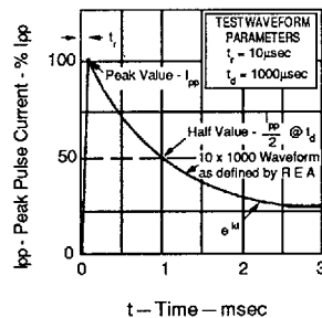
FIGURE 2 — Pulse Waveform
