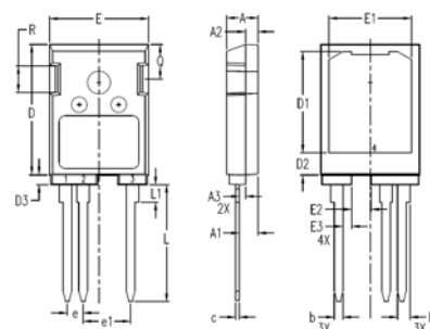
TO-247PLUS-HV Outline
