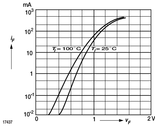
Fig. 1 Forward characteristics
