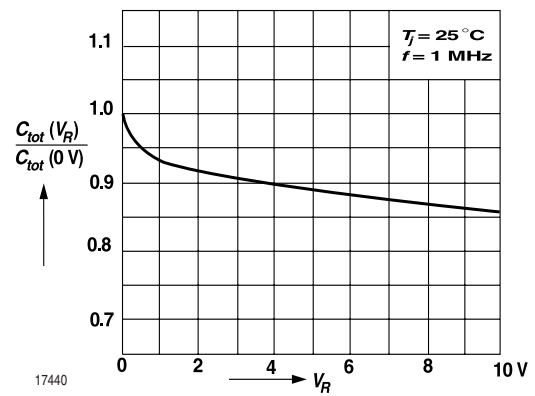
Fig. 4 Relative Capacitance vs. Reverse Voltage
