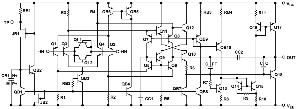
Figure 4. Simplified Schematic
