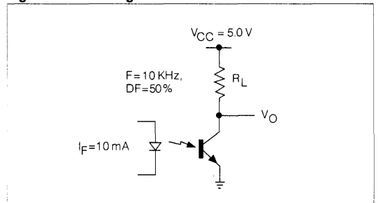
Figure 14. Switching Schematic
