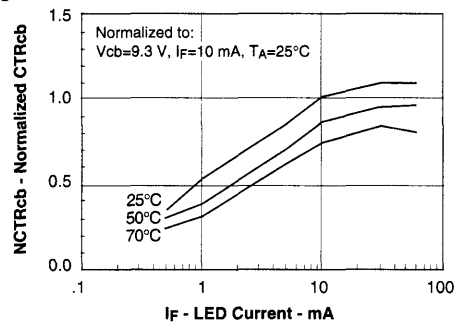
Figure 9. Normalized Photocurrent vs. I_F and Temp.
