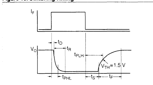
Figure 13. Switching Timing
