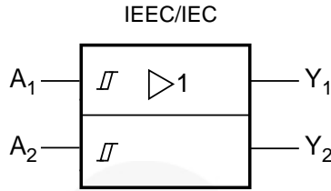
Figure 1. Logic Symbol
