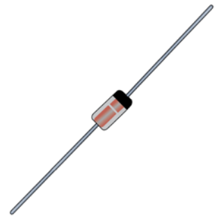
DO-7 Package
