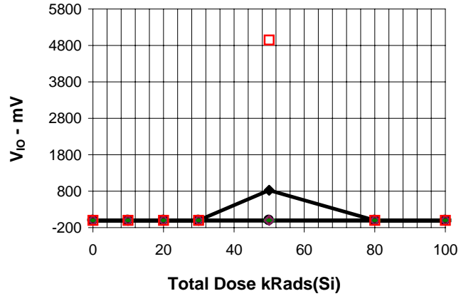
V_{IO} ; V_+=30V , V_{CM}=28V , AMP 2 vs Total Dose
