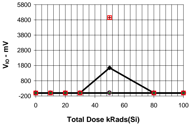
V_{IO} ; V_+=5V , V_{CM}=0V , AMP 1 vs Total Dose
