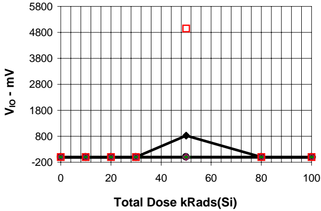
V_{IO} ; V_+=30V , V_{CM}=28V , AMP 1 vs Total Dose
