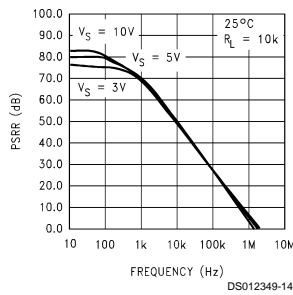
Pos PSRR vs Frequency
