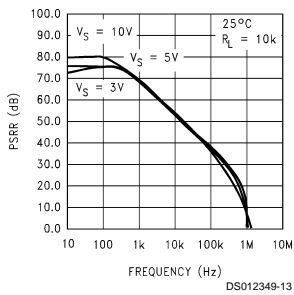
Neg PSRR vs Frequency
