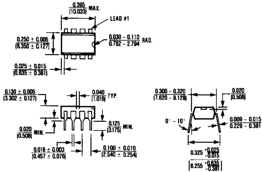
8 Lead Plastic DIP \theta_{JA} = 120^{\circ}\text{C/W} \theta_{JC} = 70^{\circ}\text{C/W}
