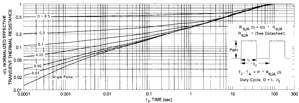
Figure 16. TO-92, 2N7000 Transient Thermal Response Curve.
